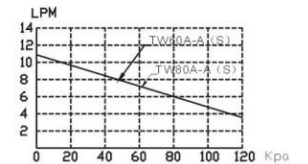
Characteristic Curve
