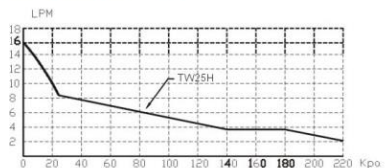
Characteristic Curve
