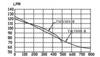
Characteristic Curve
