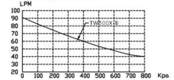
Characteristic Curve
