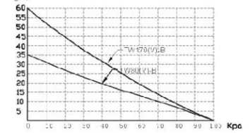
Characteristic Curve
