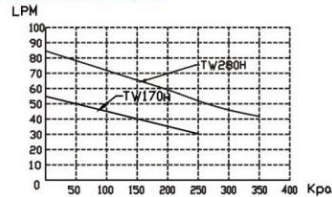
Characteristic Curve
