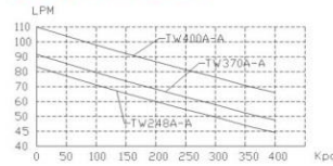
Characteristic Curve
