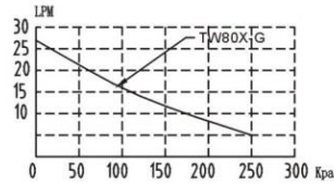
Characteristic Curve
