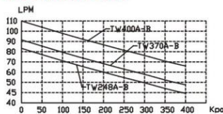
Characteristic Curve
