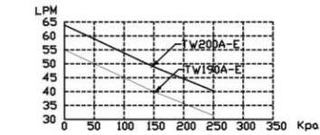
Characteristic Curve
