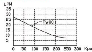
Characteristic Curve
