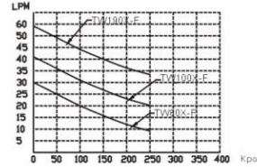
Characteristic Curve
