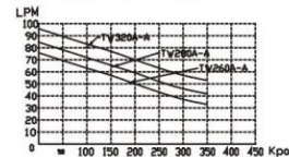
Characteristic Curve
